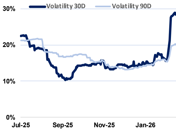
Figure 7: SET Index Volatility 30Day and 90Day
